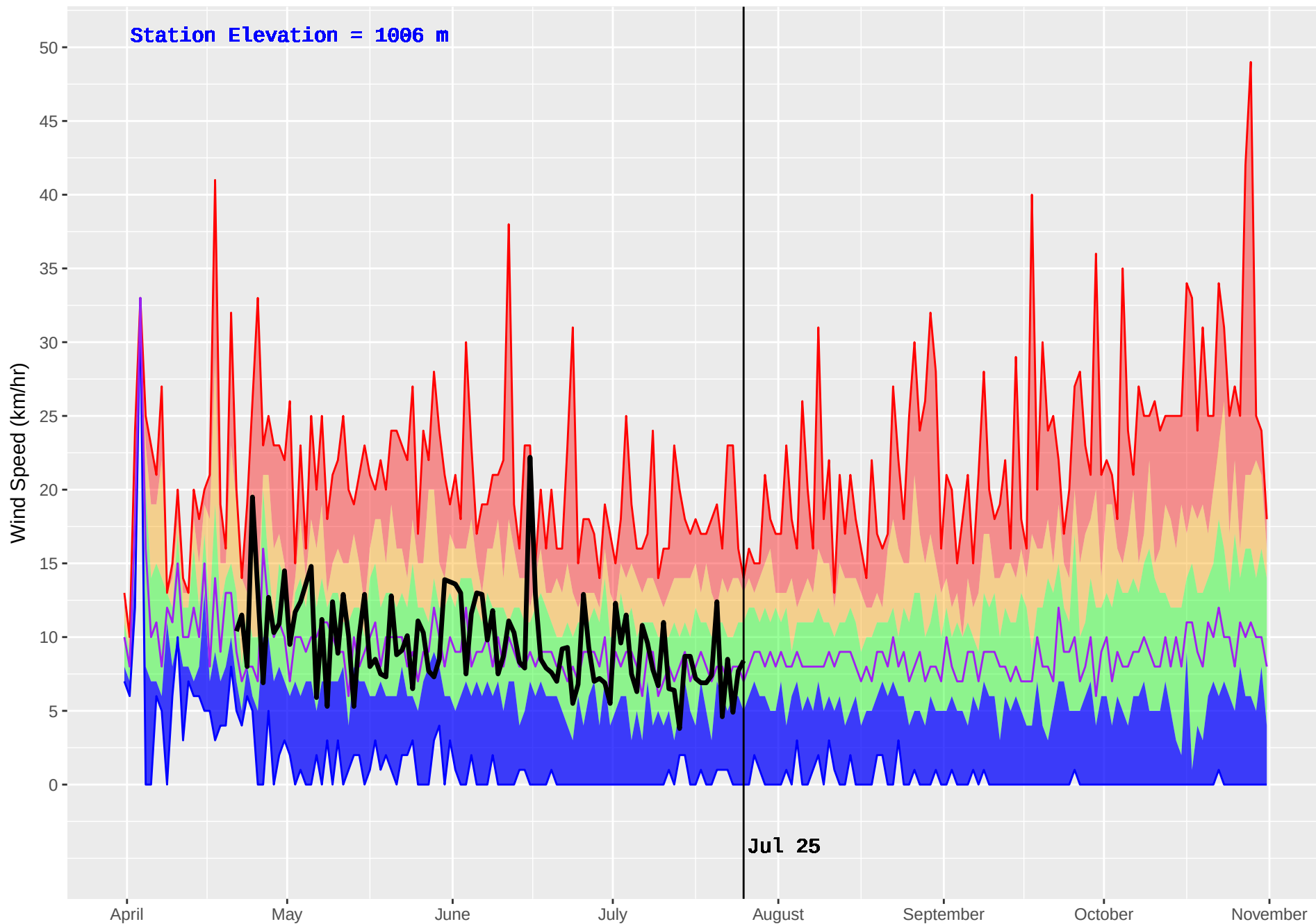
BENSON (228) : Historical (1987–2016) and Current (2017) Noon Wind Speed
