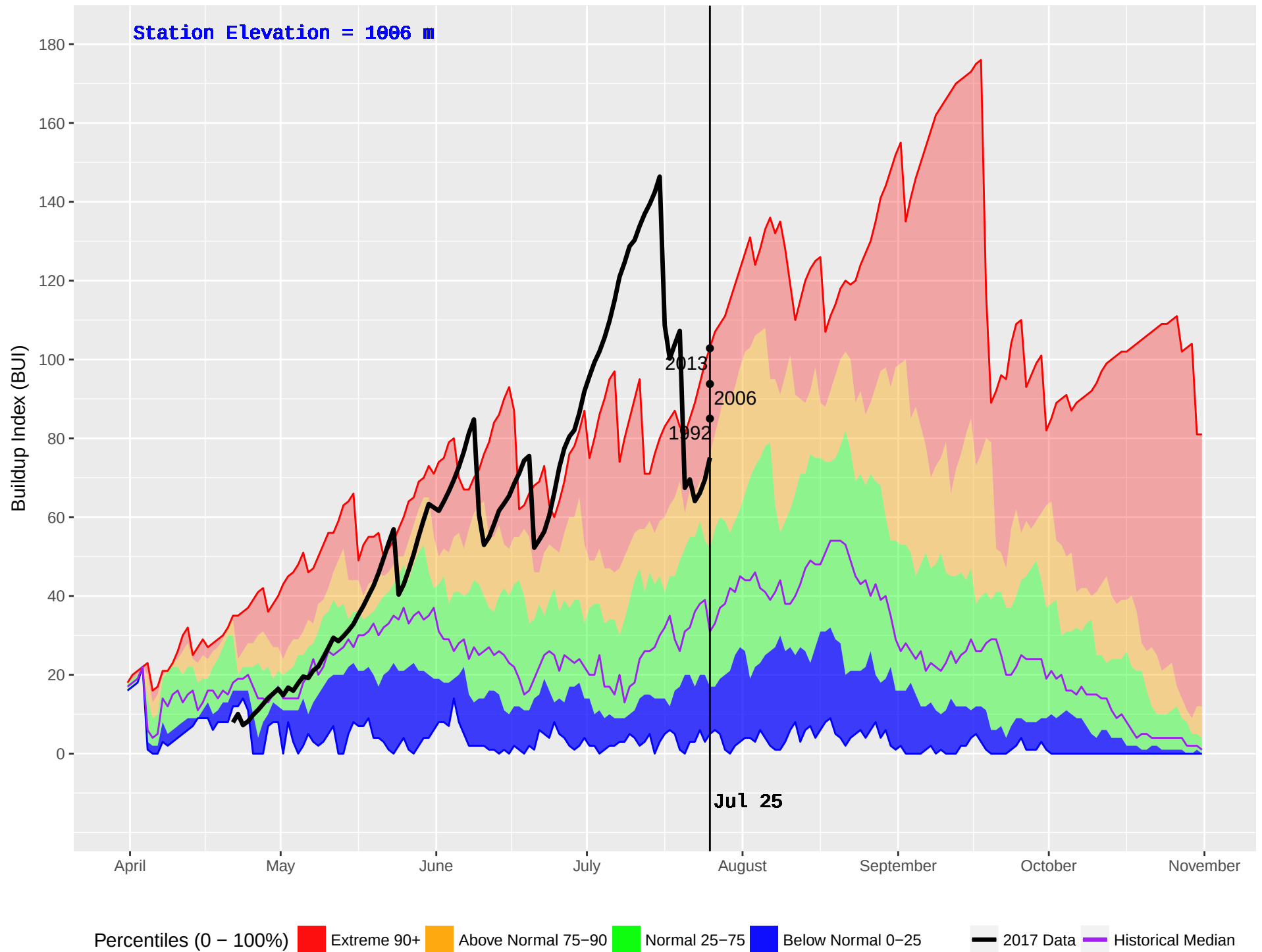
BENSON (228) : Historical (1987–2016) and Current (2017) Noon Buildup Index (BUI)
