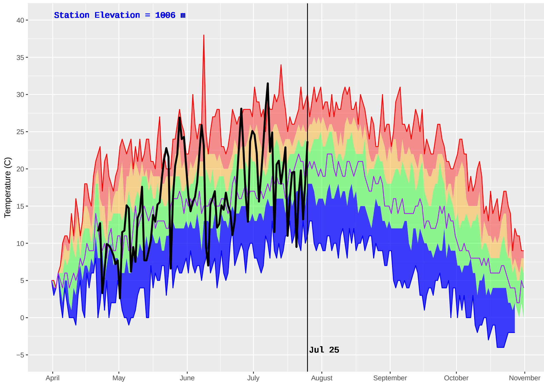
BENSON (228) : Historical (1987–2016) and Current (2017) Noon Temperature
