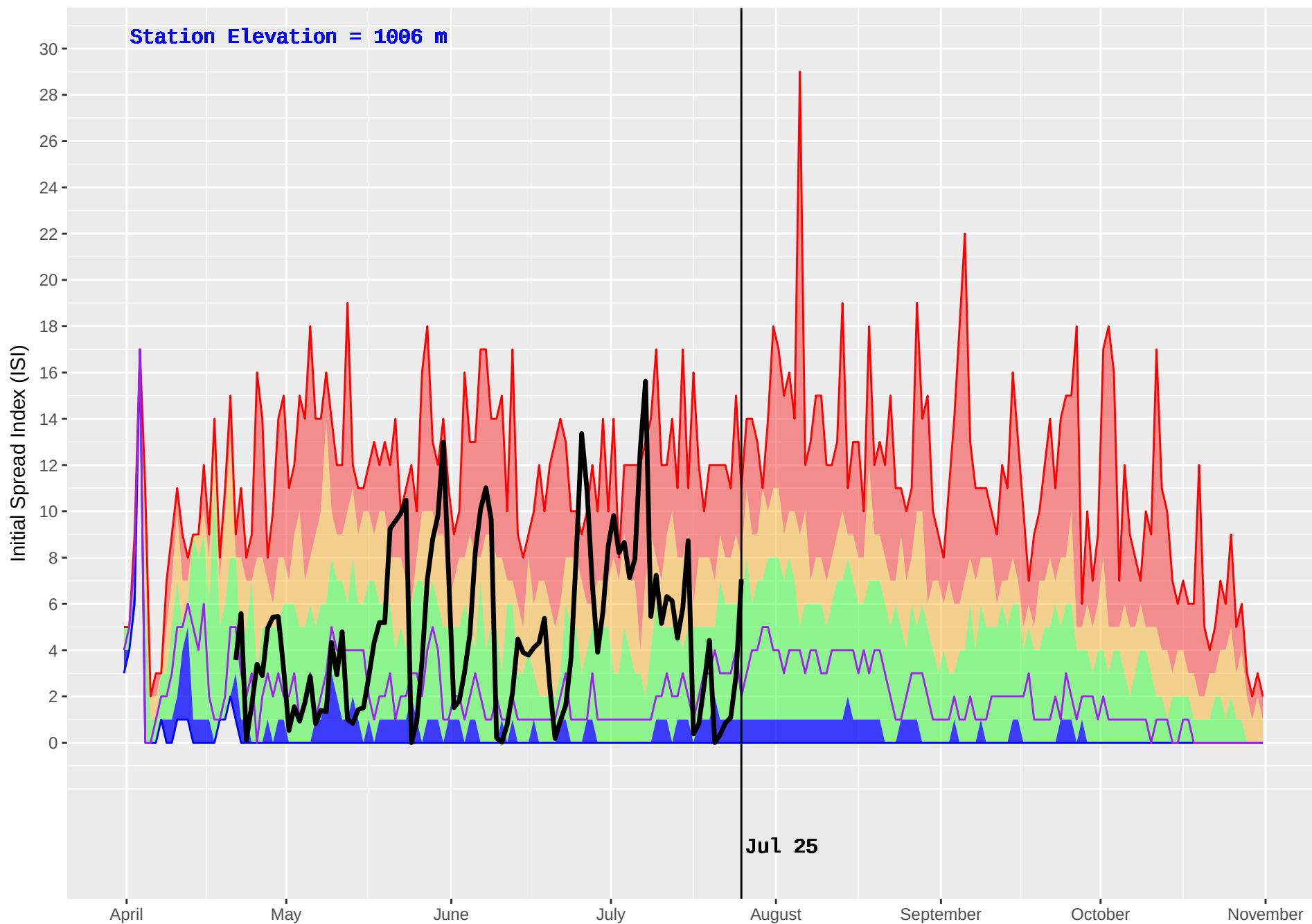
BENSON (228) : Historical (1987–2016) and Current (2017) Noon Initial Spread Index (ISI)
