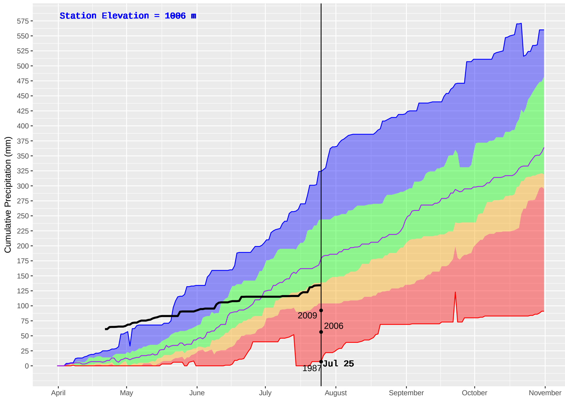
BENSON (228) : Historical (1987–2016) and Current (2017) Noon Cumulative Precipitation
